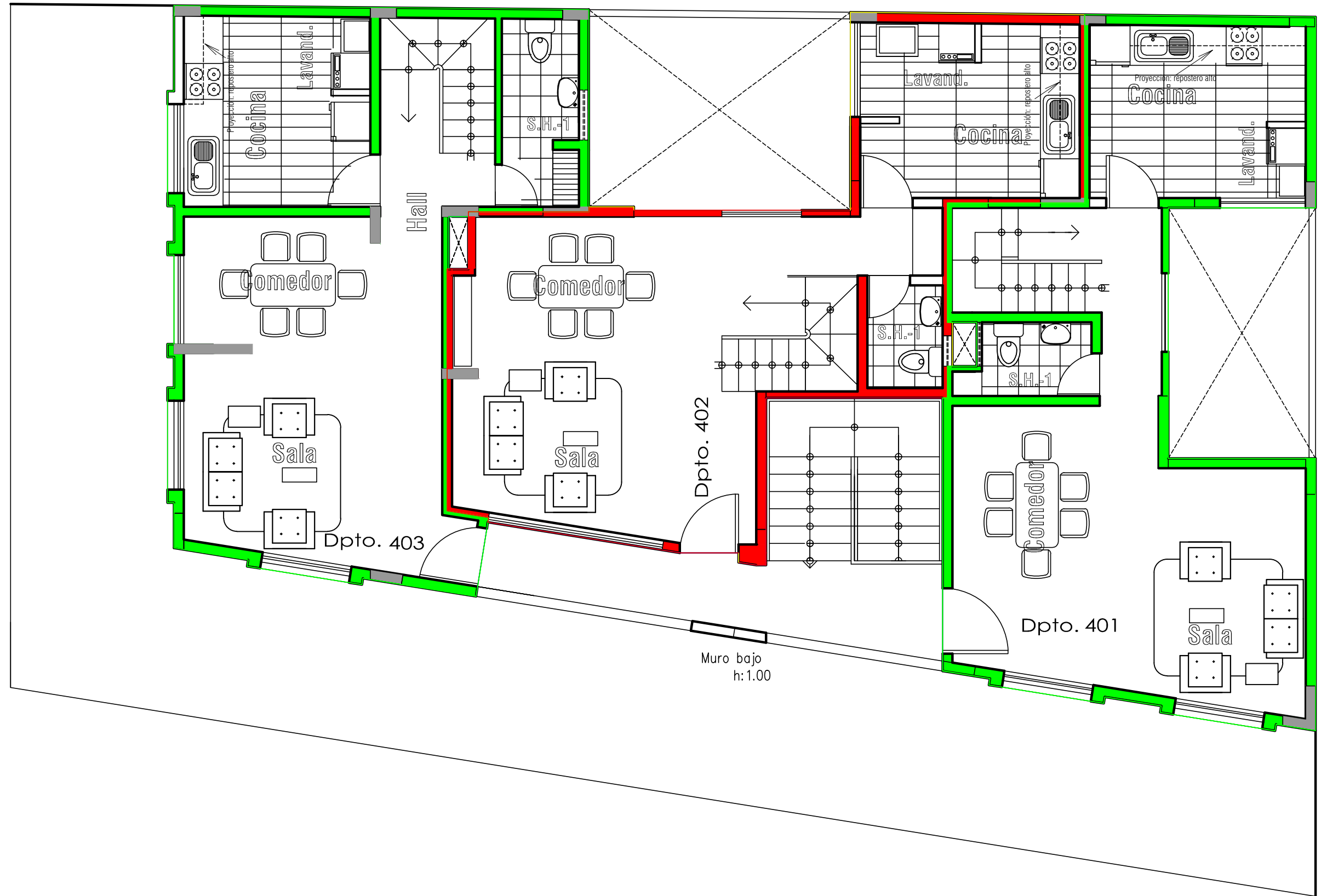
PLANTA: 4to PISO (Duplex)
